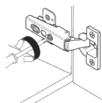
Side adjustment
